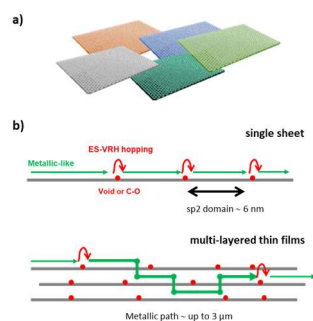
Figure 1: a) Scheme of RGO assemblies. b) Scheme of the charge transport on single sheet and on thin film. The green arrow is the metallic like transport (no hopping) and the red arrow next to the border defects is the ES-VRH hopping.
