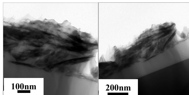
Fig. 1 – Cross sectional TEM micrographs of Graphite Platelet LDPE sample.
