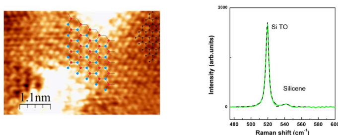
Fig. 1: Left: STM image (10.0 nm x 6.3 nm), obtained after Si IML deposition on HOPG at RT. A stick-and-ball model, representing Si atoms in a honeycomb and low buckled silicene arrangement, is superimposed as a guide for the eye. Note the presence of small, 1 nm high, silicon clusters (white regions). Right: Raman spectrum of the sample shown in the left panel.
