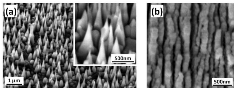
Fig1: SEM micrograph of SiC surfaces treated using a) fluorine based reactive ion etching and b) femtosecond laser, respectively.
