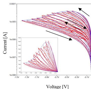
Fig. 1- Hysteron and I-V curves for Ti/ h BN/Cu. Fig. 3- Hysteron and I-V curves for Ti/MLG/ h BN/MLG/Au.
