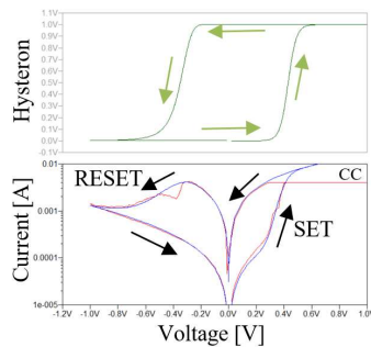
Fig. 1- Hysteron and I-V curves for Ti/ h BN/Cu. Fig. 3- Hysteron and I-V curves for Ti/MLG/ h BN/MLG/Au.
